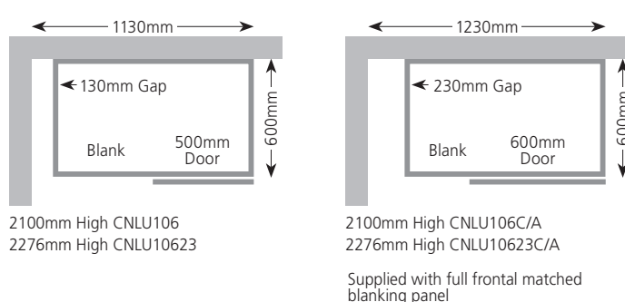
Corner Larder Cabinet
