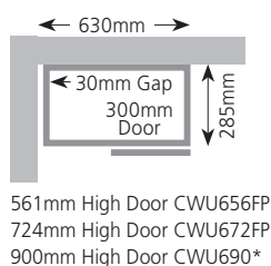
600mm Corner Wall Cabinet
