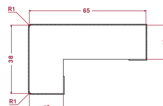
Square Universal Cornice and Pelmet CORPEL30F (Alta Gloss, Alta Matt, Minnesota, Plaza & Quadra only)
