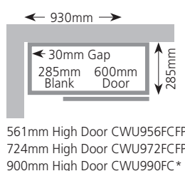
900mm Corner Wall Cabinet
